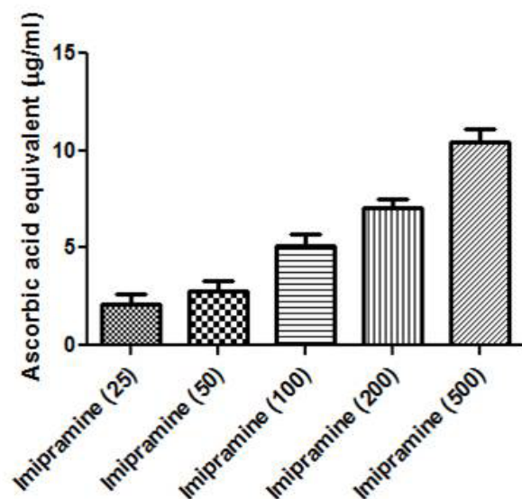
Figure 6: Graphical representation of determination of cupric ion reducing antioxidant capacity of imipramine by CUPRAC assay.
