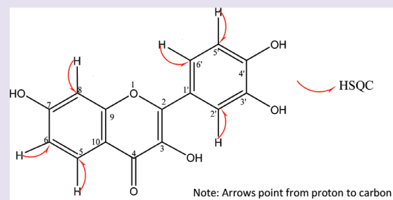
Figure 2: The key HSQC correlations of Fisetin
