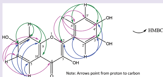
Figure 1: The key HMBC correlations of Fisetin
