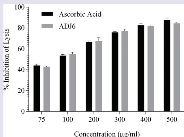
Figure 2a: RBC Membrane Stabilization Assay (n=3)
