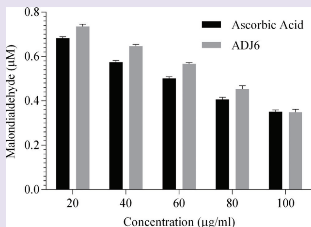
Figure 2c: Estimation of Malondialdehyde (n=3)
