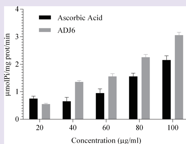
Figure 2d: Na + K + ATPase Assay (n=3)
