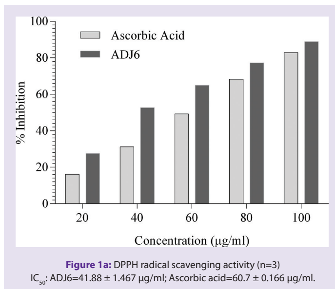
Figure A: Antioxidant Analysis of ADJ6
