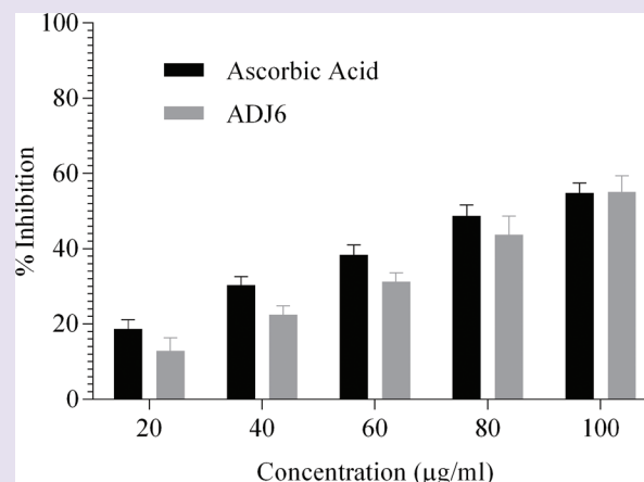
Figure 2b: Inhibition of Lipid Peroxidation (n=3)
