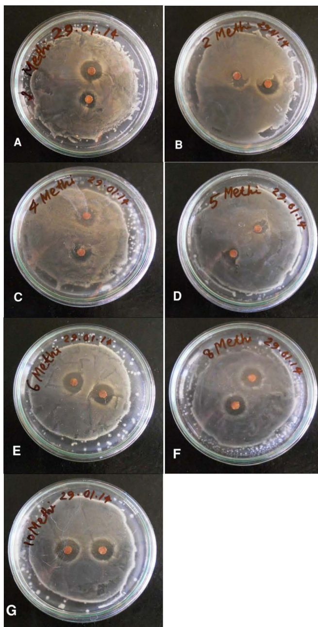
Figure 1: Zone of inhibition of T. foenum-graecum essential oil against (A) B. subtilis (B) S. lutea (C) X. campestris , (D) K. pneumoniae , (E) E. coli , (F) P. denitrificans and (G) P. vulgaris
